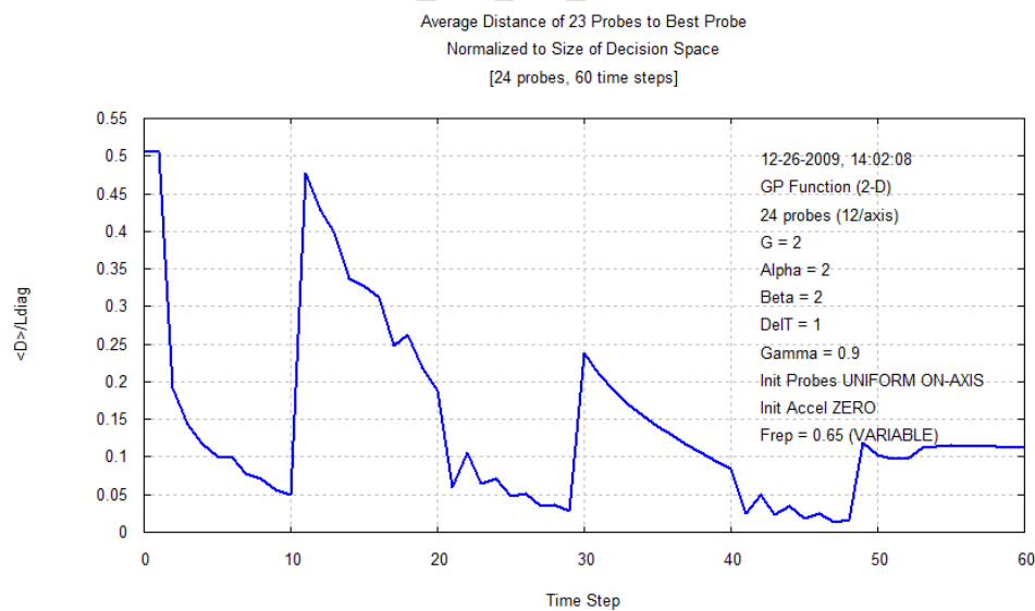
250 251 Fig. 8. Evolution of GP Function D_{avg}
