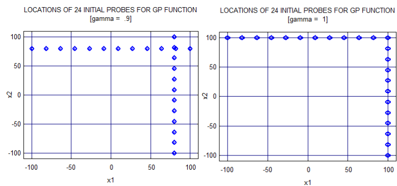
Fig. 5. GP Best Run Initial Probe Distributions
