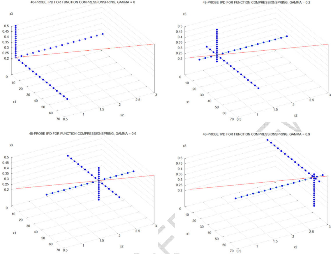
Fig. 6. Example of a 3D Probe Line IPD
